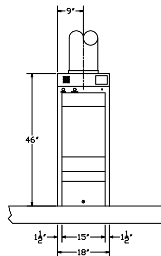
FRONT ELEVATION
